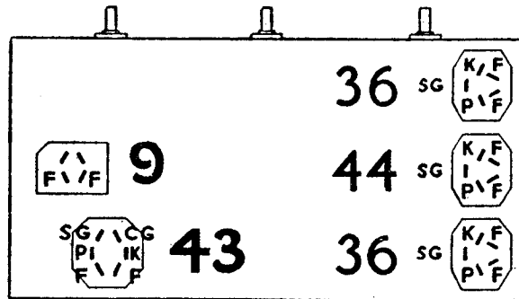
Fig. 1—Tube Sockets, Under Side of Chassis
